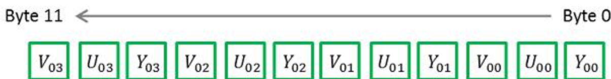
Figure 4. Packing format for YCbCr8.
