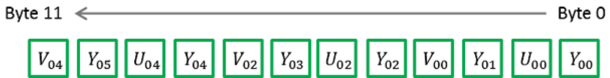
Figure 7. Packing format for YCbCr422_8.
