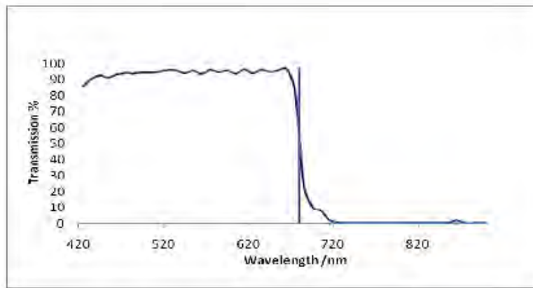
Figure 4.3: IR filter transmittance graph
