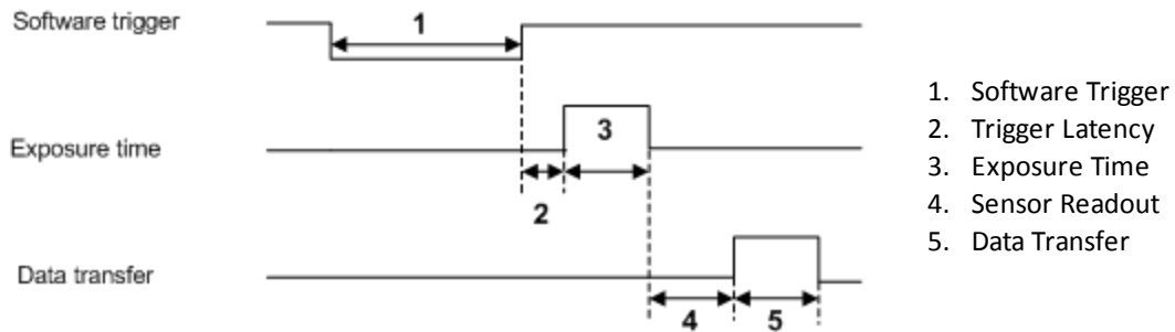
Figure 7.11: Software trigger timing
