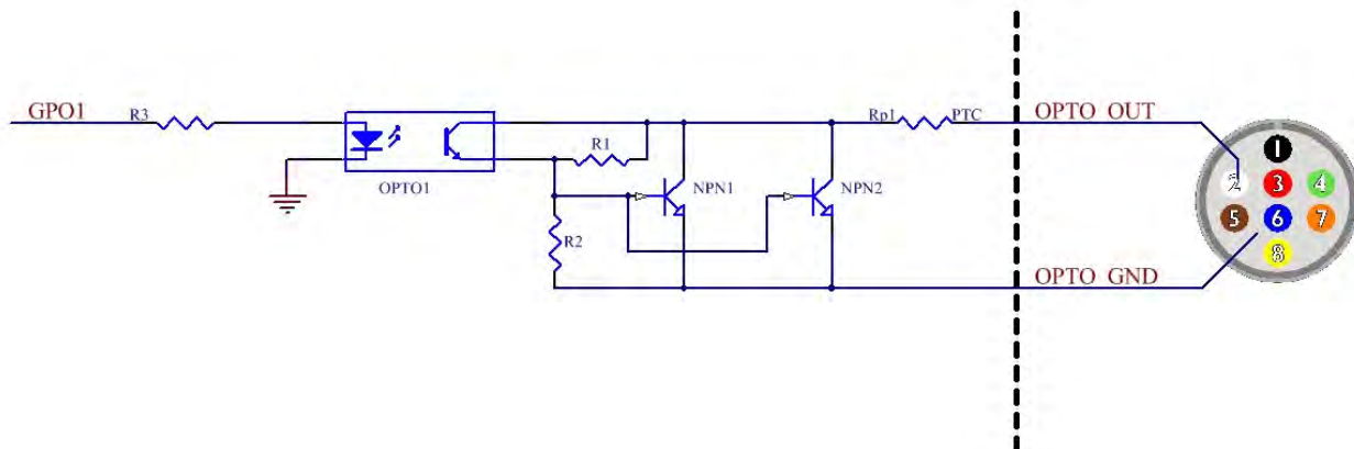
Figure 6.3: Opto-isolated output circuit
