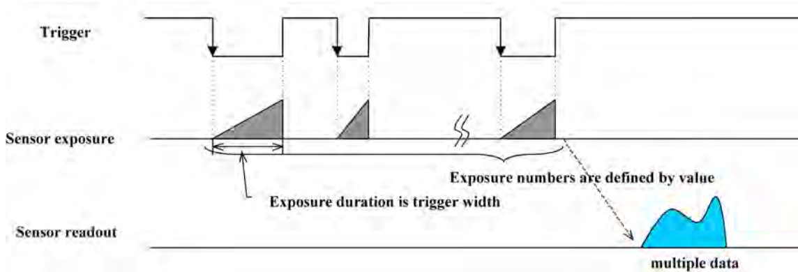
Figure 7.5: Trigger Mode 5 (“Multiple Exposure Pulse Width Mode”)
