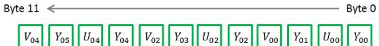
Figure 9. Packing format for YCbCr422_8.
