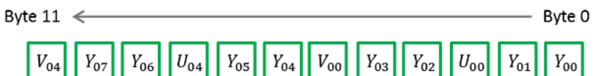
Figure 10. Packing format for YCbCr411_8 .
