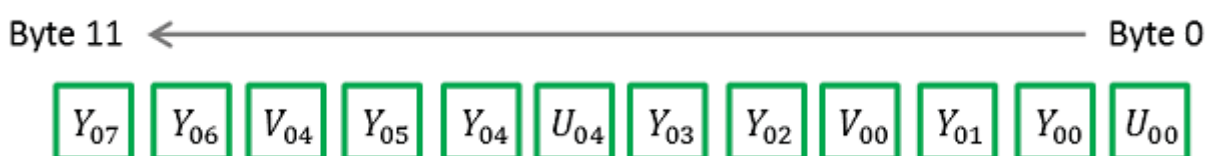
Figure 12. Packing format for YUV411Packed .
