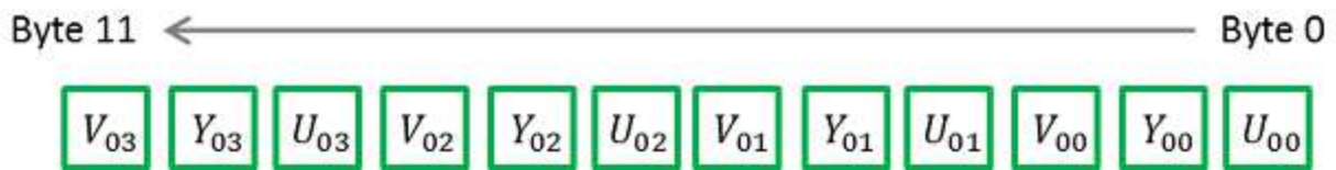
Figure 5. Packing format for YUV444Packed.
