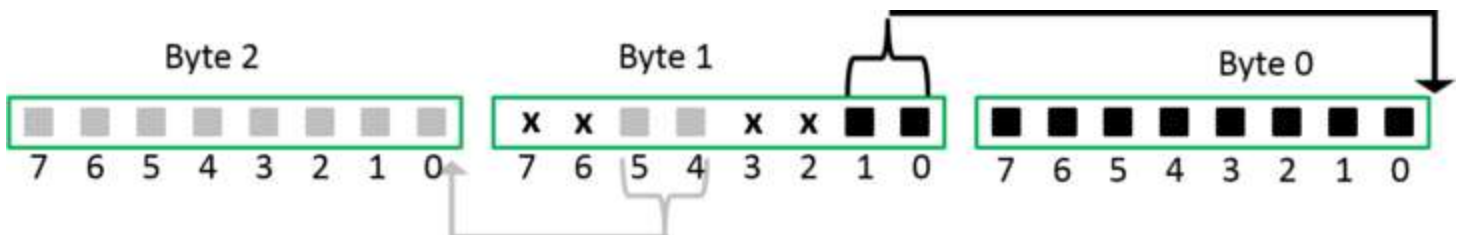
Figure 2. Packing two 10-bit pixels into three bytes.
