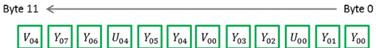
Figure 12. Packing format for YCbCr411_8.
