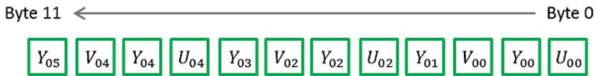
Figure 8. Packing format for YUV422Packed .
