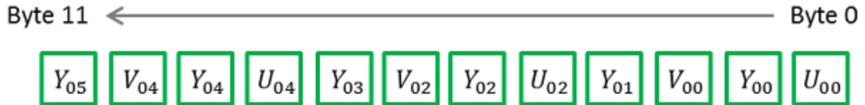
Figure 10. Packing format for YUV422Packed.
