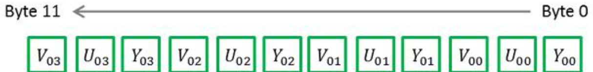
Figure 4. Packing format for YCbCr8.
